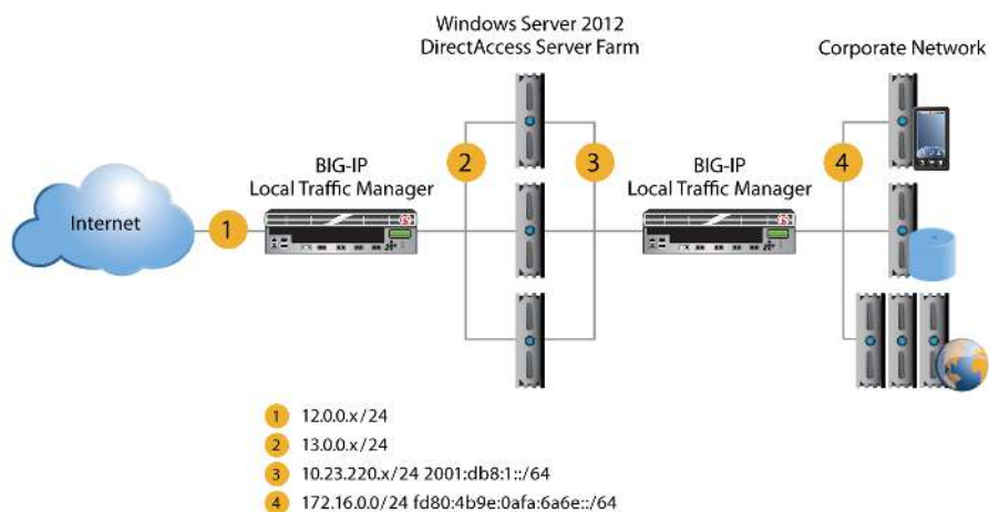
Figure 4: A layered deployment with dual interface routing
