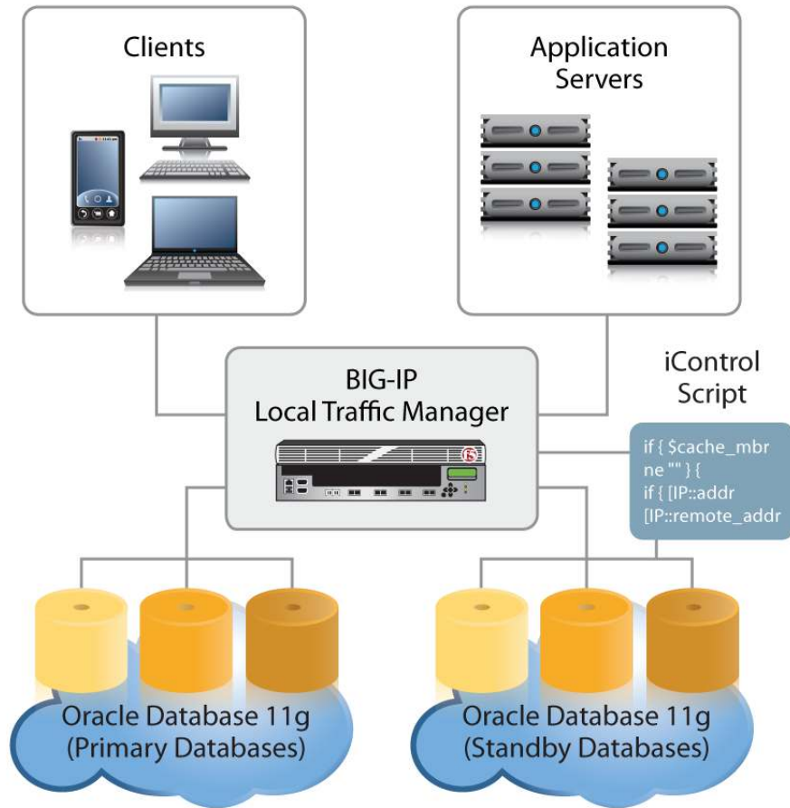
Figure 2: BIG-IP LTM extends FAN notifications to all applications, not just those built on the Oracle JVM.
