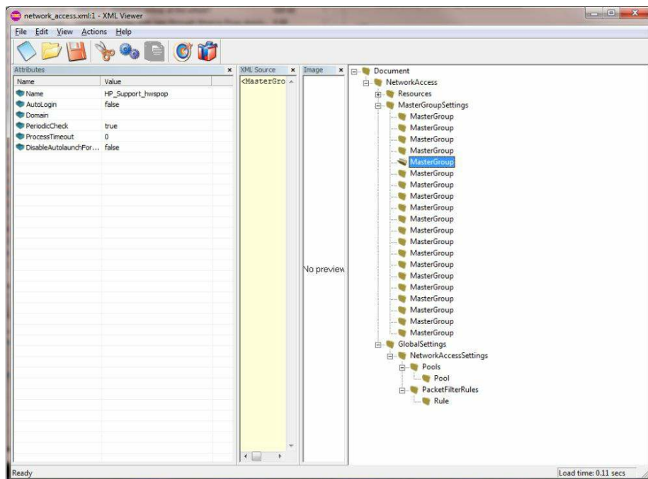
Figure 3: Exported FirePass XML file view.
