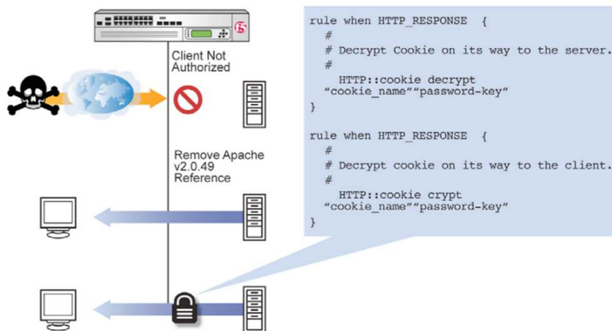
Figure 2: Encrypt/Decrypt Cookies
