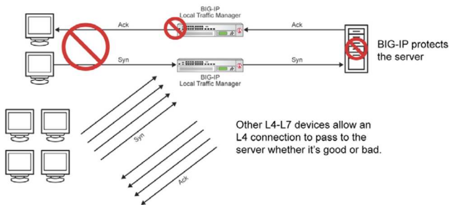
Figure 3: SYN CHECK example
